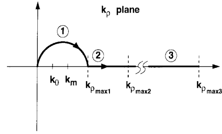
Fig. 3. Three-level GPOF sampling paths.
